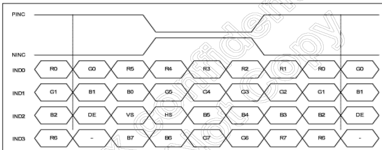
8-bit LVDS input
